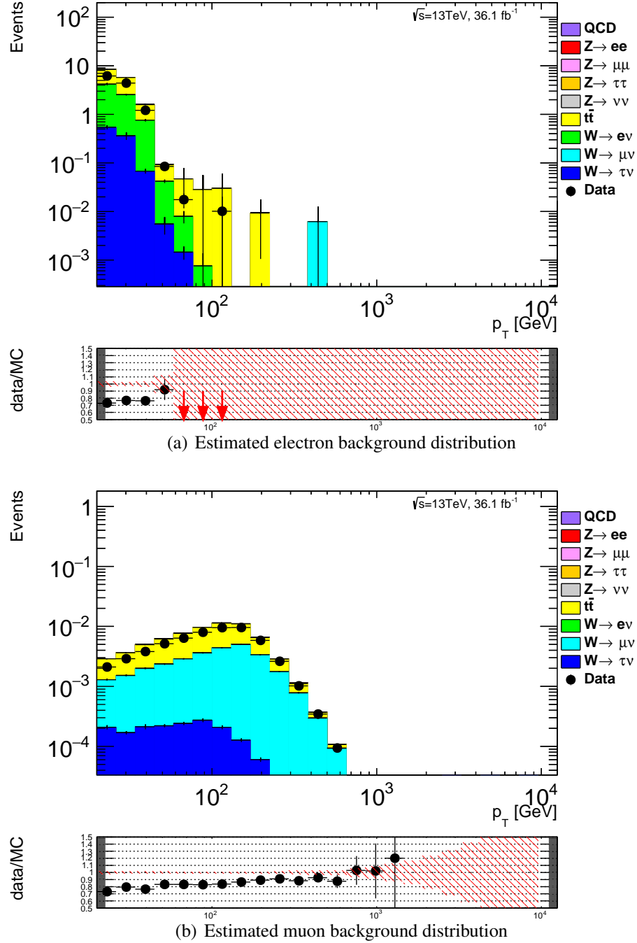
Figure 8.11: The estimated electron and muon background distributions before smearing. Various MC standard model processes are shown in the stacked histogram and data in the black points. The lower plot shows the ratio of data and MC in the black points and MC statistic uncertainty is shown by the red shade.
