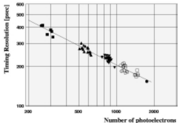
Figure 4: Timing resolution of the prototype as a function of number of observed photoelectrons.
