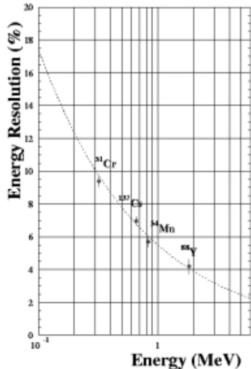
Figure 3: Energy resolution measured with gamma-ray sources as compared to the predictions (dashed line) by the simulation.
