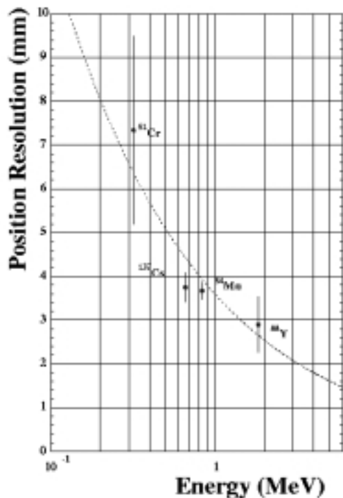
Figure 4: Position resolution measured with the prototype. The dashed line shows the prediction by the simulation.
