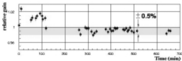
Figure 2: Time stability of PMT output monitored with scintillation light from liquid Xe activated by \alpha particles as a function of time after the vessel was filled with liquid Xe. For the first stage of monitoring the output is unstable due to unstable temperature and pressure, although it is stabilized in \pm 0.5\% after 200 to 250 minutes.
