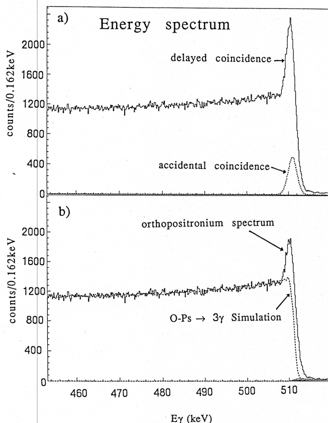
FIG. 3. (a) The photon-energy spectrum taken with the delayed and the accidental coincidences. The accidental spectrum is normalized by the widths of the time windows. (b) The delayed-coincidence spectrum (histogram) after the accidental contribution is subtracted. The dotted line, almost indistinguishable from the data below 508 keV, shows the simulated spectrum from the 3\gamma decay of o -Ps.
