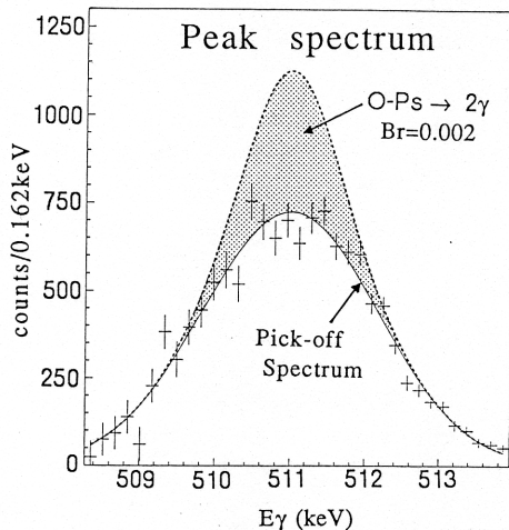
FIG. 4. The enlarged view of the peak at 511 keV after subtracting the simulated 3\gamma contribution. The solid curve shows the shape of measured pickoff spectrum normalized to data by total number of events under the peak. The shaded area indicates the shape and the magnitude of the peak from the o -Ps \rightarrow 2\gamma decay with a branching ratio of 0.2%.
