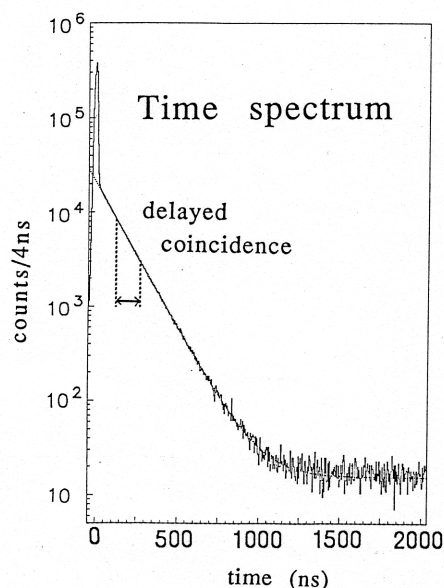
FIG. 2. A time-difference distribution between the scintillator and the germanium signals.
