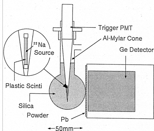
FIG. 1. Setup of the experiment. Circular inset: A magnified view of the source region.
