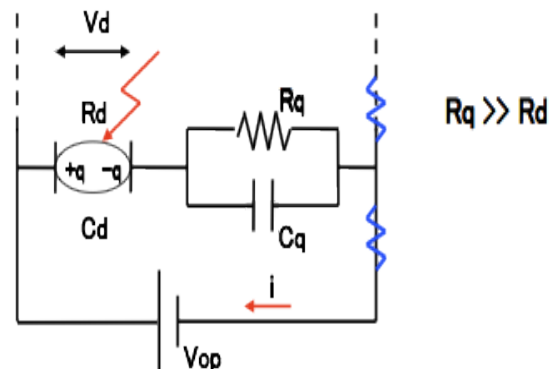
< Equivalent circuit of MPPC by Otono et al. >
