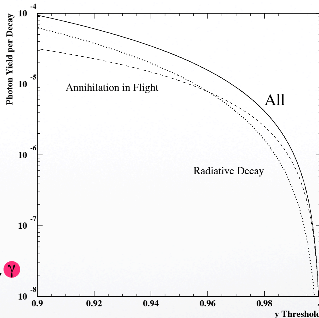
Spectrum of background gamma
