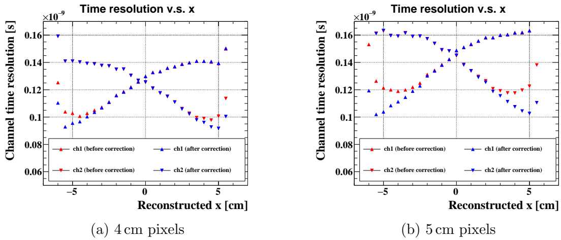
Figure 9.2: x hit position dependence of the channel time resolution. The red and blue makers show the position dependence before and after the time offset correction respectively.
