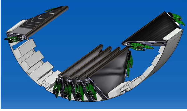
Figure 3.8: The design of the MEG DCH [20]. Only a fraction of the modules are depicted.
