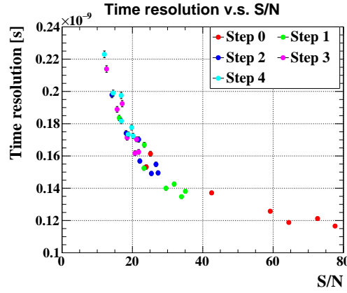
Figure 7.2: Relation between the S/N and the time resolution. The bias voltage scan data at 30 °C with different damage levels is used.
