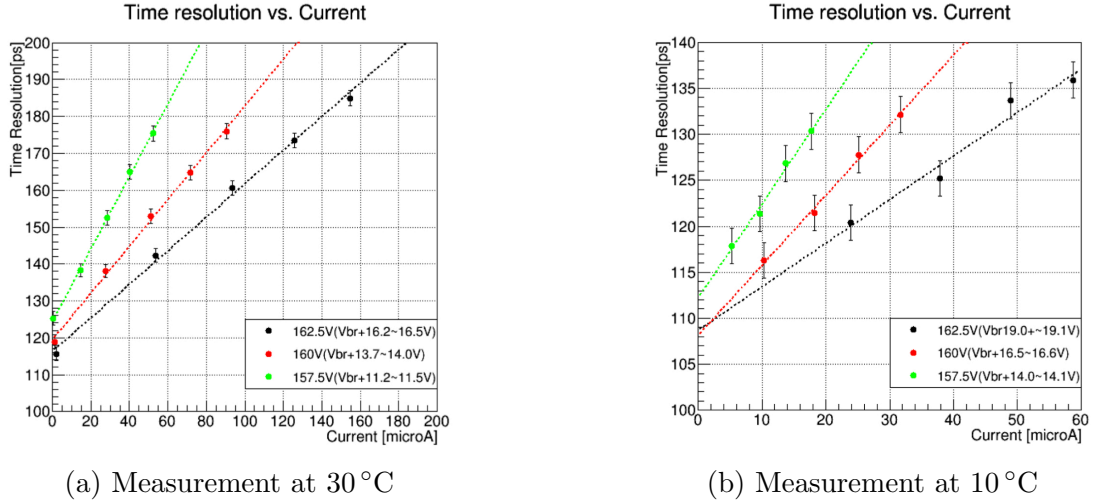
Figure 4.19: The single-pixel time resolution as a function of the readout current [54]. Different points in the same color show measurements at different damage levels.
