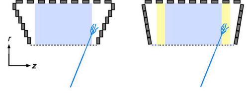
Figure 3.25: MEG (left) and MEG II (right) layout of the PMTs viewed in an r - z section [27].
