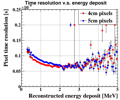
Figure 9.6: Energy deposit dependence of the pixel time resolution.
