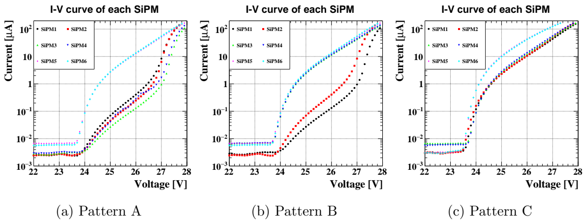
Figure 6.18: I-V curves of SiPMs used in each damage pattern at 10 °C. SiPMs with less damage are labeled with younger numbers.
