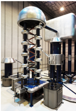
Figure 3.17: The Cockcroft-Walton pre-accelerator [30].
