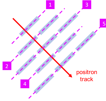
Figure 4.10: Definition of the geometry ID for clustering.
