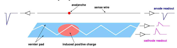
Figure 3.10: A schematic view of the vernier pad method [17].
