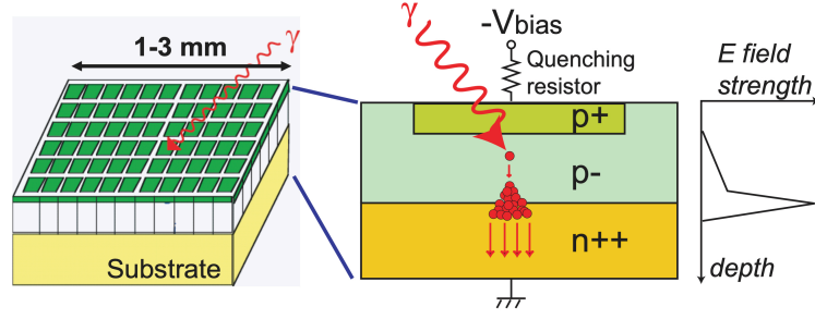
Figure 4.5: Schematic view of how a SiPM works [45].
