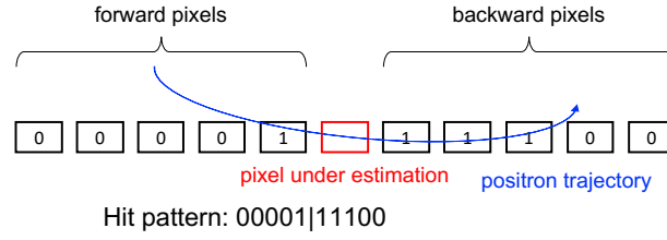
Figure 4.11: A schematic diagram of y_{\text{hit}} estimation from the cluster hit pattern.
