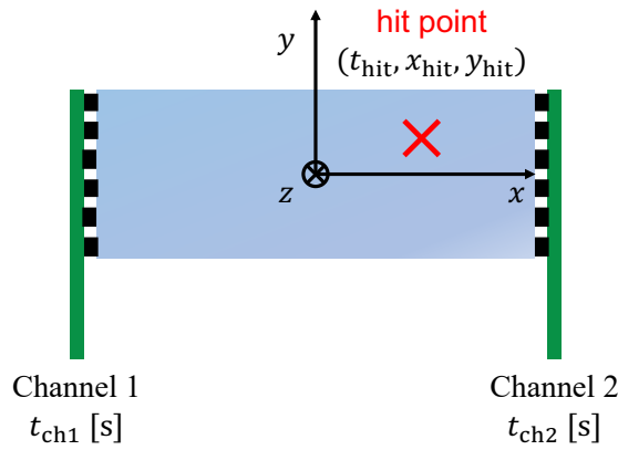
Figure 4.9: Definition of the local coordinates in a pixel.
