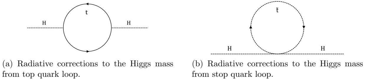
Figure 2.3: One-loop corrections to the Higgs mass.
