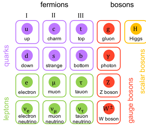
Figure 2.1: Elementary particles in the SM.
