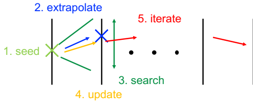
Figure 4.12: A schematic diagram of the principle of the KF.
